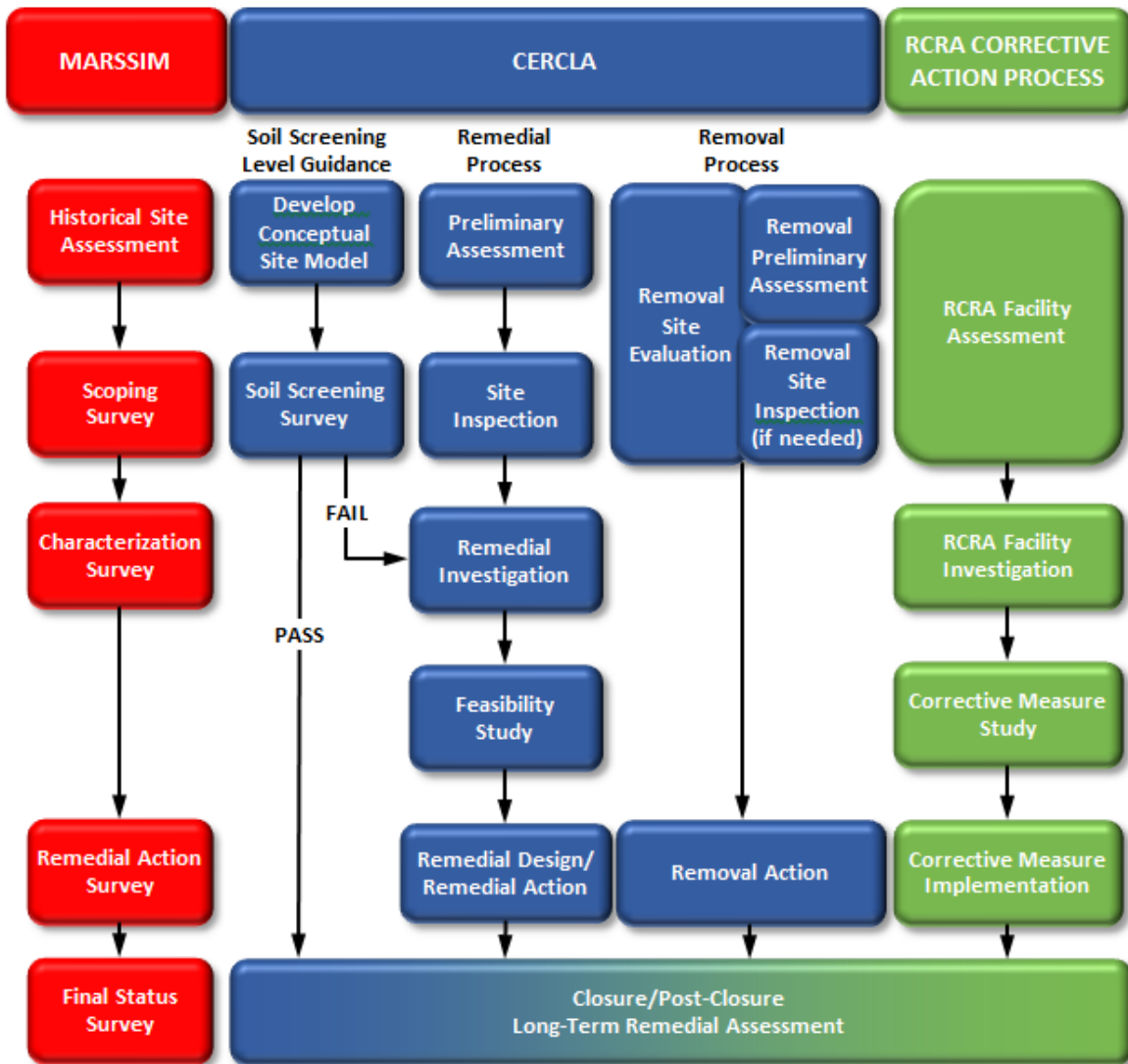
Figure 2 – Comparison of MARSSIM, CERCLA, and RCRA Processes
